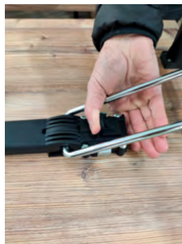
Handles to unlock the legs under the tops
