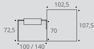
Top view (right hand DDA (1) )
